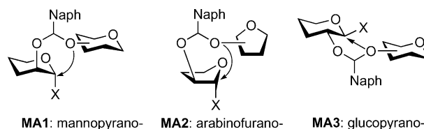
Figure 2. 1,2- cis induction via mixed acetals.
