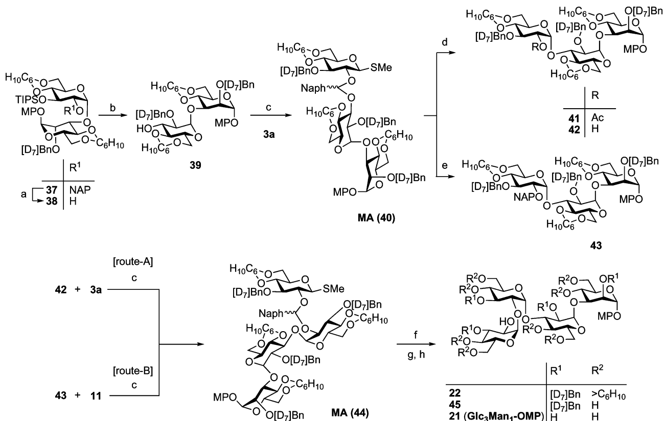
Scheme 5. Synthesis of Glc 3 Man 1 -OMP 21 ; reagents and conditions: (a) DDQ, NaHCO 3 , (CH 2 Cl) 2 , 86%; (b) [D 7 ]BnBr, NaH, DMF; then TBAF, THF, 75% in two steps; (c) DDQ, MS (4 Å), CH 2 Cl 2 , 96% (2.72:1) ( 40 ), 47% (2.33:1) ( 44 ) from 42 (route A), 97% (3.43:1) ( 44 ) from 43 (route B); (d) (i) MeOTf, DTBMP, MS (4 Å), (CH 2 Cl) 2 ; (ii) Ac 2 O pyridine, 85% ( 41 ); (iii) NaOMe, MeOH, 88% ( 42 ); (e) MeOTf, DTBMP, (TMS) 3 SiH, MS (4 Å), (CH 2 Cl) 2 , 76% ( 43 ) and 6% ( 42 ); (f) (i) MeOTf, DTBMP, (TMS) 3 SiH, CH 2 Cl 2 ; (ii) DDQ, NaHCO 3 , (CH 2 Cl) 2 , 77%; (g) TFA; (h) Pd(OH) 2 , H 2 , MeOH/H 2 O (2:1), quant. in two steps.
