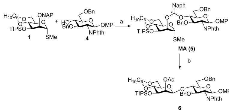
Scheme 1. NAP-IAD for \beta -mannopyranoside; reagents and conditions: (a) DDQ, MS (4 Å), (CH 2 Cl) 2 , room temp., quant. (single isomer); (b) (i) MeOTf, DTBMP, (CH 2 Cl) 2 , r.t.; (ii) Ac 2 O, pyridine, 90% (only \beta -isomer).
