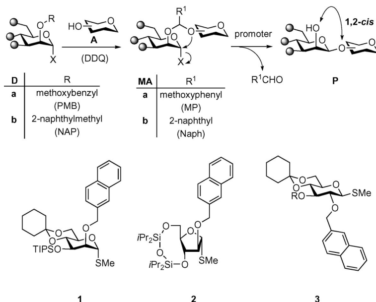
Figure 1. Intramolecular aglycon delivery using NAP ether protected glycosyl donors.
