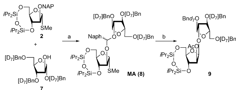
Scheme 2. NAP-IAD for \beta -arabinofuranoside; reagents and conditions: (a) DDQ, MS (4 Å), (\text{CH}_2\text{Cl})_2 , quant. (3.40:1); (b) (i) MeOTf, DTBMP, (\text{CH}_2\text{Cl})_2 , r.t.; (ii) TFA; (iii) \text{Ac}_2\text{O} , pyridine, 77% ( \beta -9).
