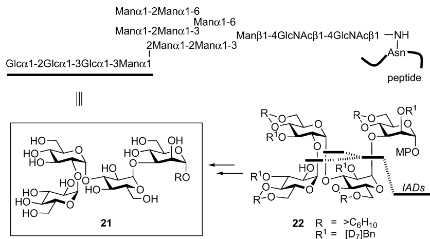
Figure 3. Triglycosylated high-mannose-type N -glycan.
