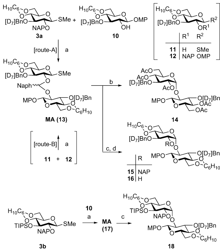
Scheme 3. NAP-IAD for \alpha -glucosides; reagents and conditions: (a) DDQ, MS (4 Å), \text{CH}_2\text{Cl}_2 , room temp., 96% (3.18:1) from 3a (route A); 93% (1:4.17) from 11 (route B); 84% (>10:1) from 3b ; (b) (i) MeOTf, DTBMP, (\text{CH}_2\text{Cl})_2 , r.t.; (ii) TFA; (iii) \text{Ac}_2\text{O} , pyridine, 72% ( \alpha -14); (c) MeOTf, DTBMP, (\text{TMS})_3\text{SiH} , (\text{CH}_2\text{Cl})_2 , room temp., 73% ( \alpha -15) and 16% ( \alpha -16); 82% ( \alpha -18); (d) DDQ, 85% ( 16 ) in two steps from 13 .
